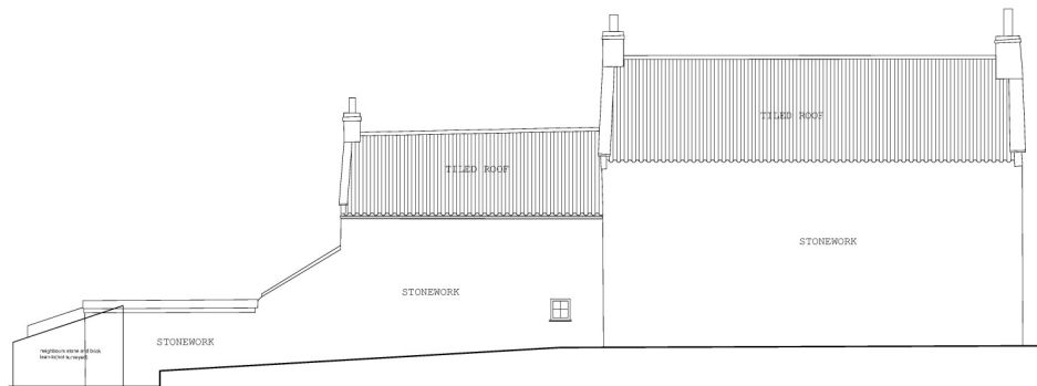
WEST ELEVATION
